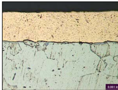
Photomicrograph of CopperPlus showing the integrity of the bond (500X)
