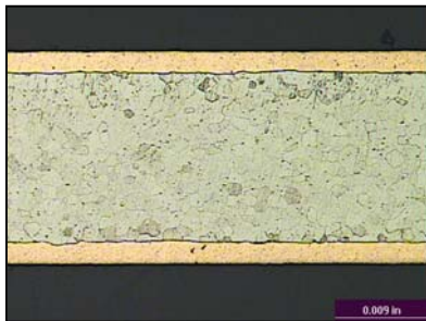
Photomicrograph of CopperPlus (100X)
